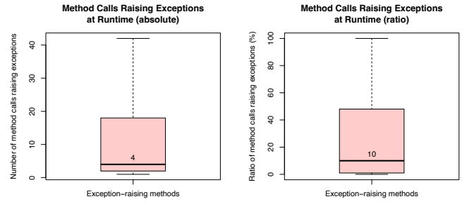
Fig. 4: Distribution of the method calls raising exceptions at runtime (absolute and relative values).
